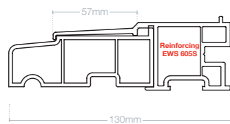
85mm A type cill AS 85
